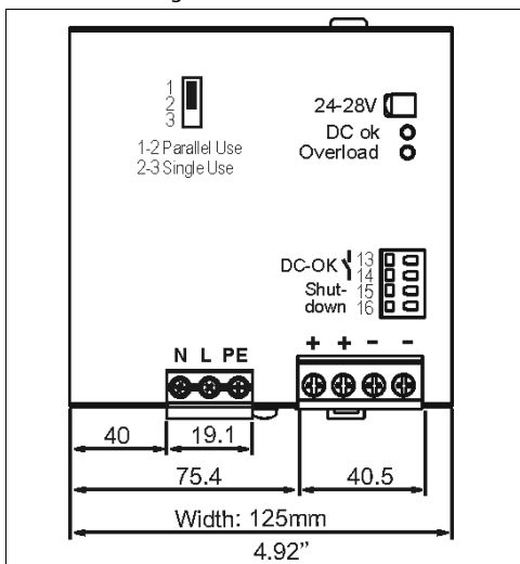
Fig. 24-1 Front view
